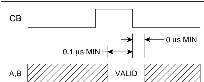
FIGURE 15. RESOLUTION CONTROL TIMING
